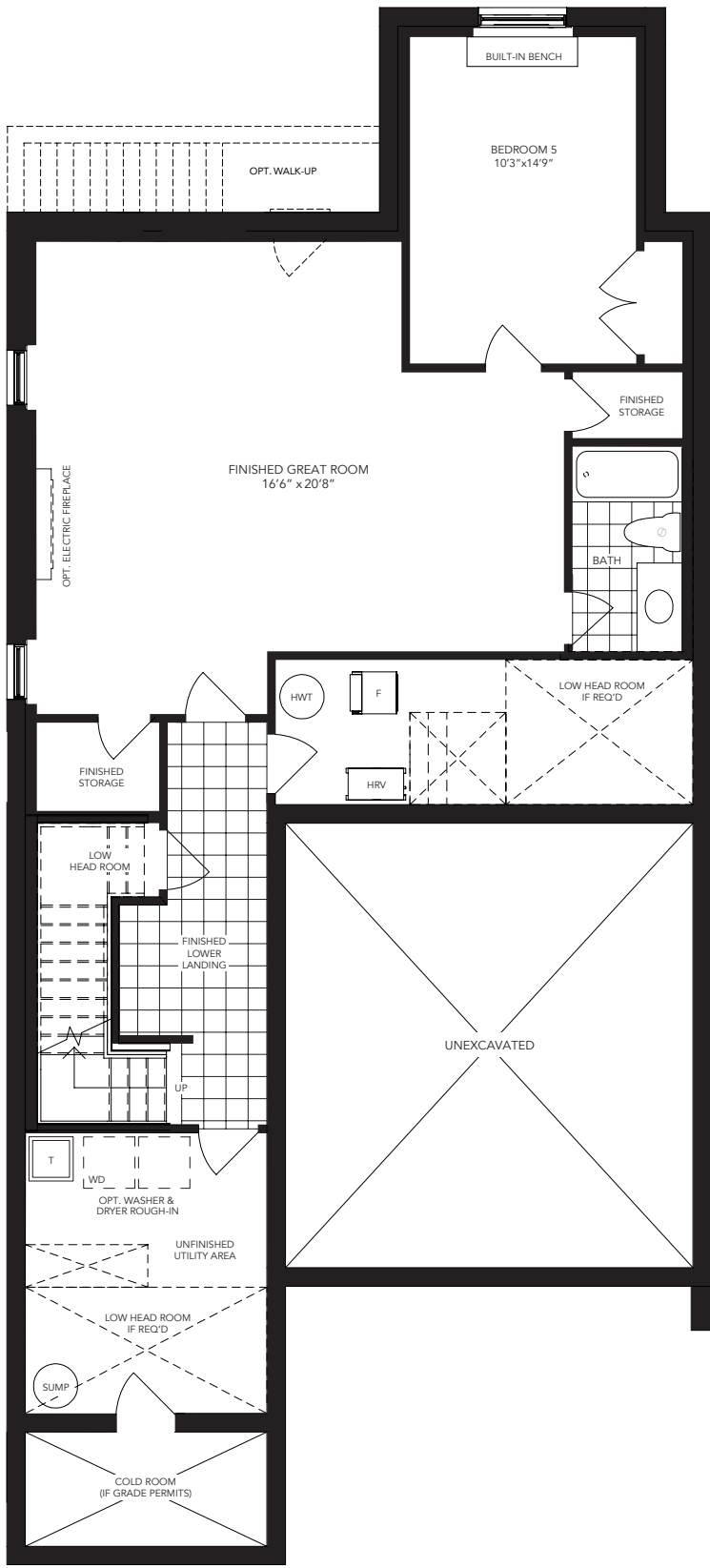
OPT. FINISHED BASEMENT - BED & BATH
