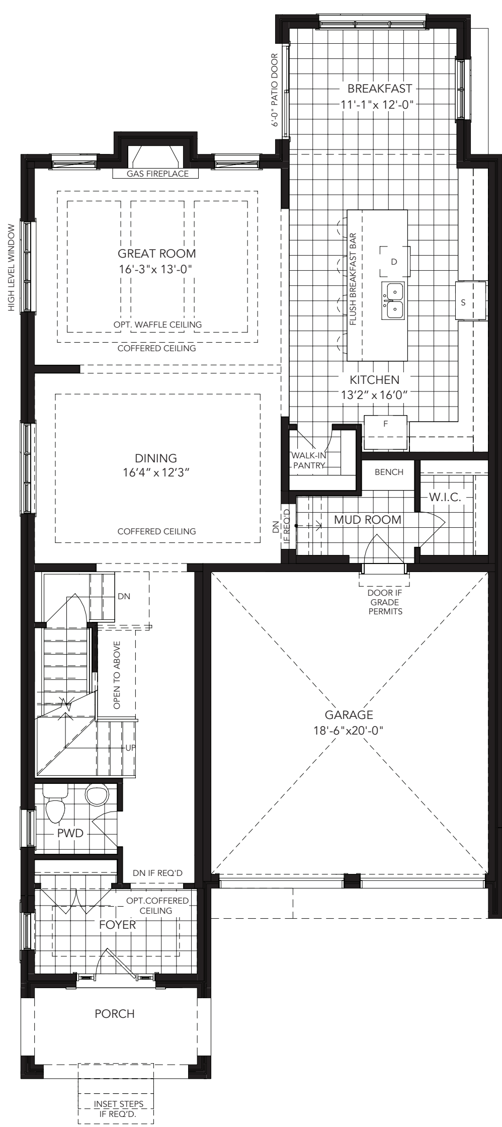
GROUND FLOOR ELEV. A
