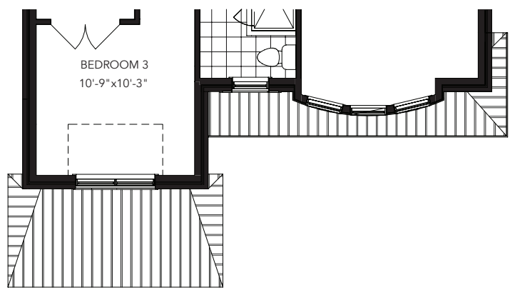
PARTIAL SECOND FLOOR ELEV. B
